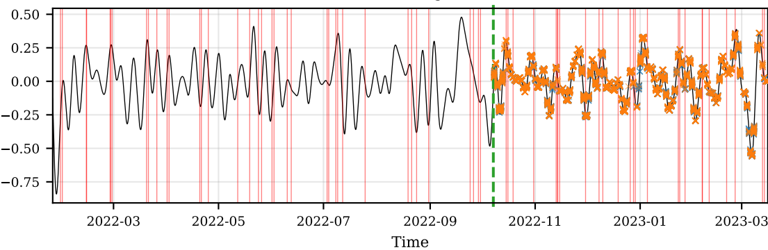
Filtered Signal
